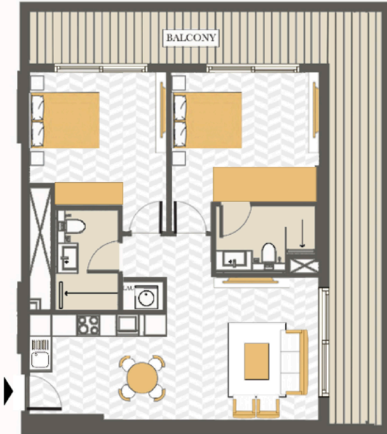
12 th – 14 th Floor Plan
